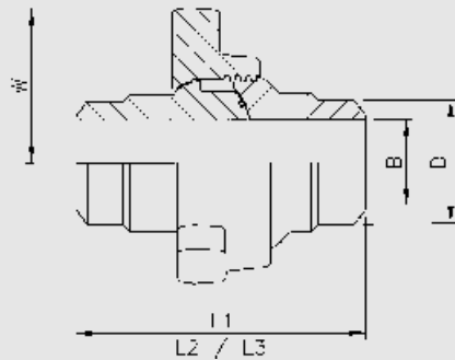
Fig 1003 Union
