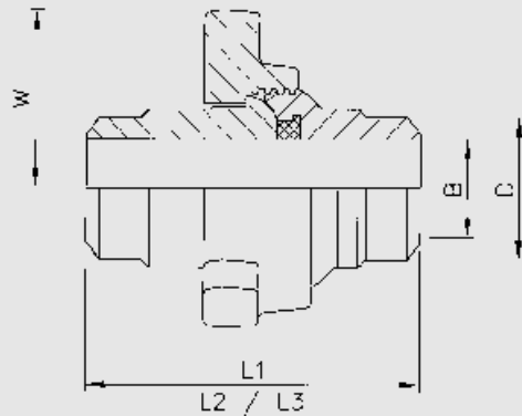
Fig 1004 Union
