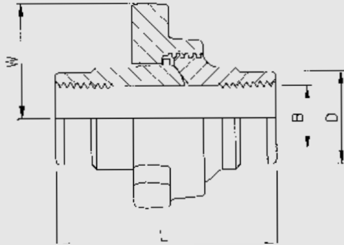
Fig 100 Union
