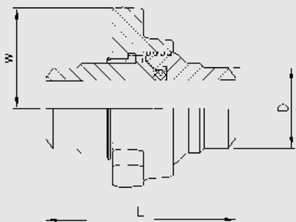
Fig 2202 Union
