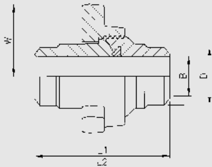
Fig 1502 Union
