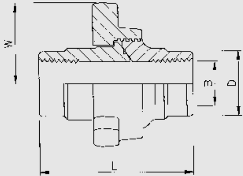
Fig 200 and 206 Union
